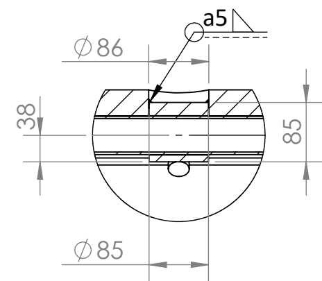
DETAIL G SCALE 2 : 15
