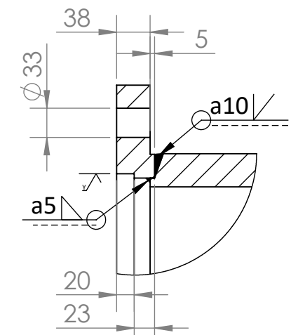
DETAIL F SCALE 1 : 6
