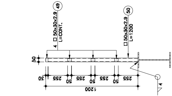
TYPICAL HANDRAIL
